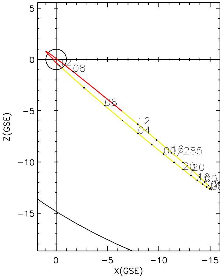
CLUSTER 2 orbit 2011 283 (10/10) 06:11 UT to 2011 285 (10/12) 12:26 UT
