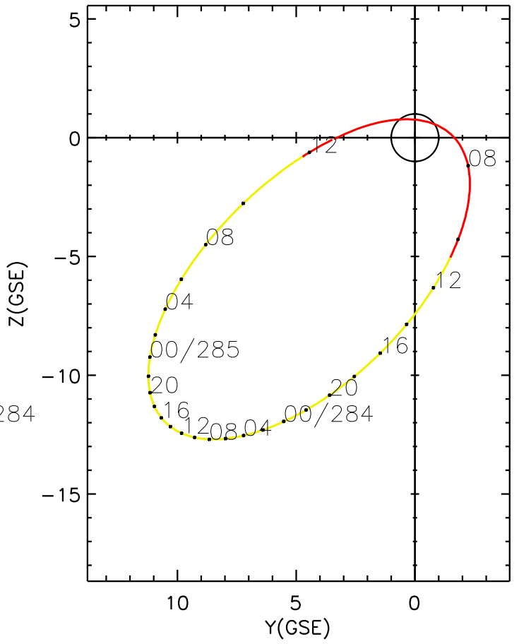
CLUSTER 2 orbit 2011 283 (10/10) 06:11 UT to 2011 285 (10/12) 12:26 UT
