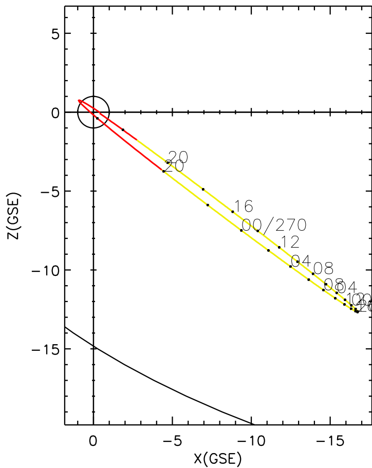
CLUSTER 2 orbit 2011 269 (09/26) 16:36 UT to 2011 271 (09/28) 22:51 UT
