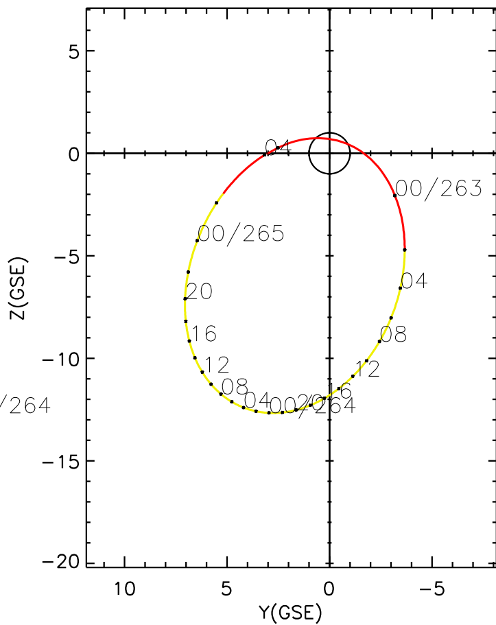
CLUSTER 2 orbit 2011 262 (09/19) 21:46 UT to 2011 265 (09/22) 04:01 UT
