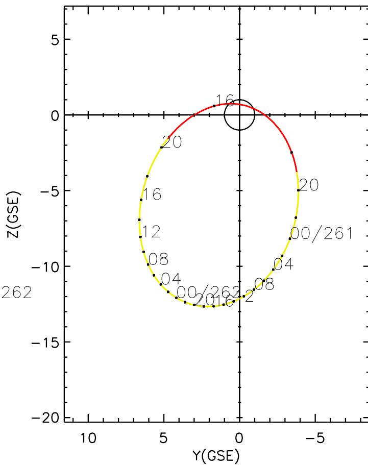
CLUSTER 2 orbit 2011 260 (09/17) 15:31 UT to 2011 262 (09/19) 21:46 UT
