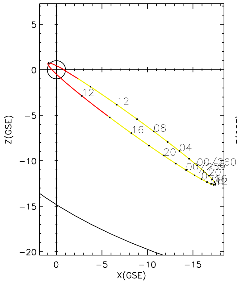
CLUSTER 2 orbit 2011 258 (09/15) 09:11 UT to 2011 260 (09/17) 15:31 UT
