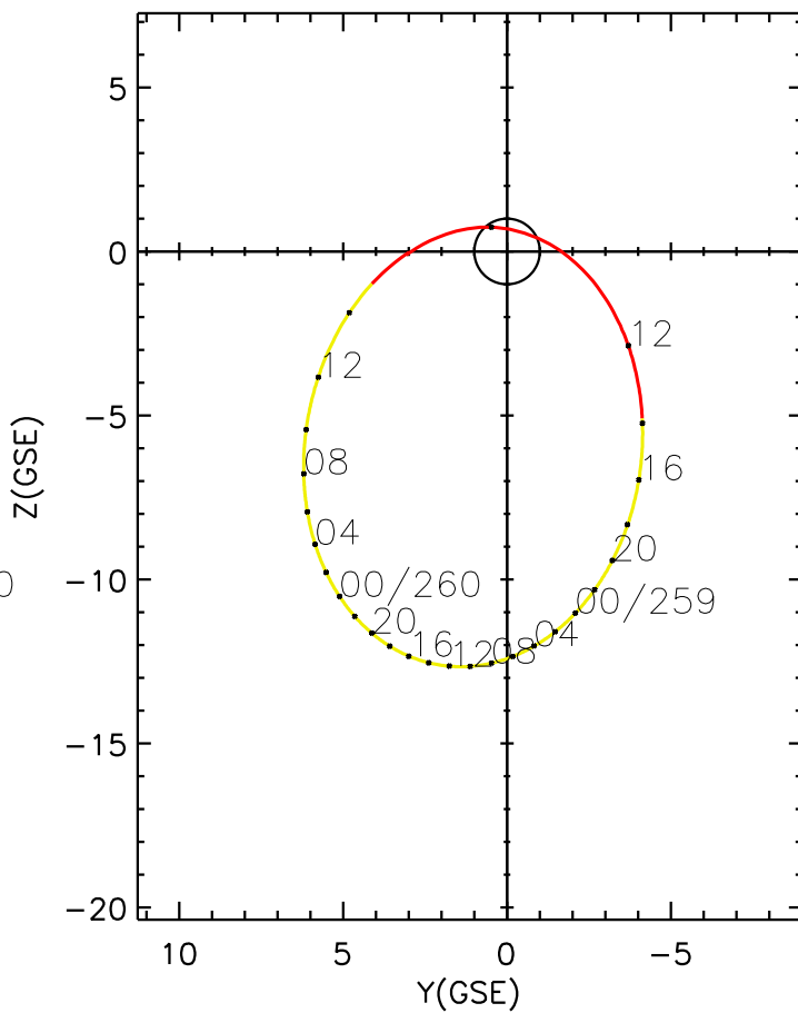
CLUSTER 2 orbit 2011 258 (09/15) 09:11 UT to 2011 260 (09/17) 15:31 UT
