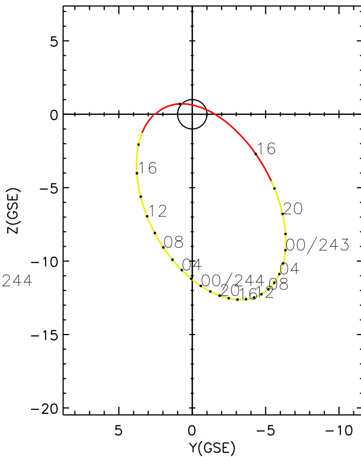
CLUSTER 2 orbit 2011 242 (08/30) 13:21 UT to 2011 244 (09/01) 19:36 UT
