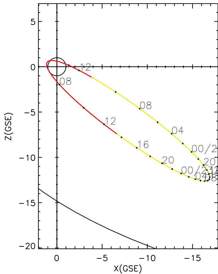
CLUSTER 2 orbit 2011 231 (08/19) 05:51 UT to 2011 233 (08/21) 12:16 UT
