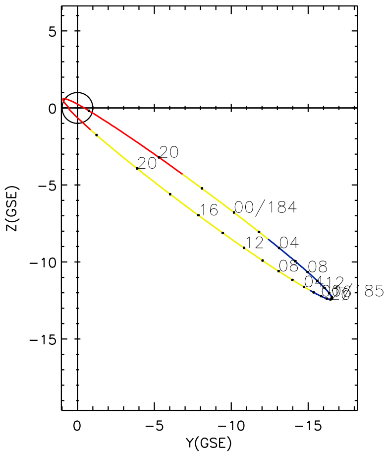
CLUSTER 2 orbit 2011 183 (07/02) 16:56 UT to 2011 185 (07/04) 23:11 UT
