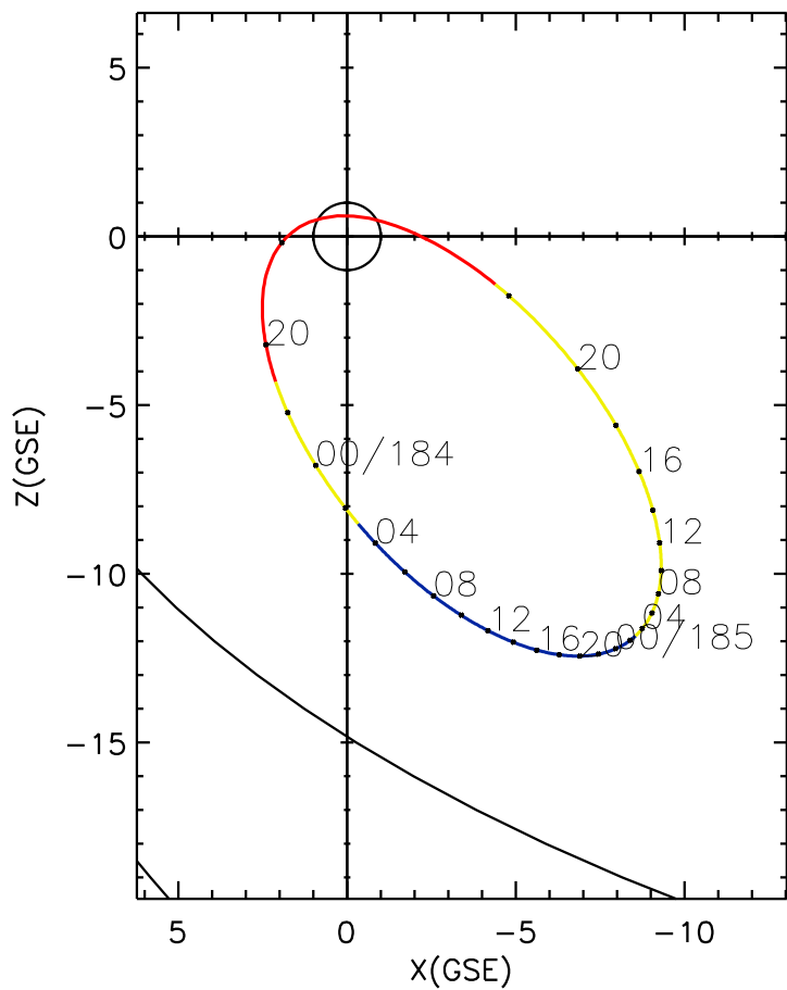
CLUSTER 2 orbit 2011 183 (07/02) 16:56 UT to 2011 185 (07/04) 23:11 UT
