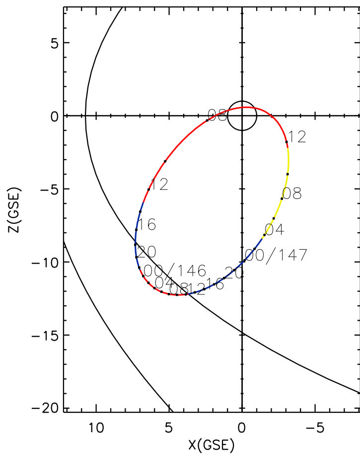
CLUSTER 2 orbit 2011 145 (05/25) 06:51 UT to 2011 147 (05/27) 13:11 UT
