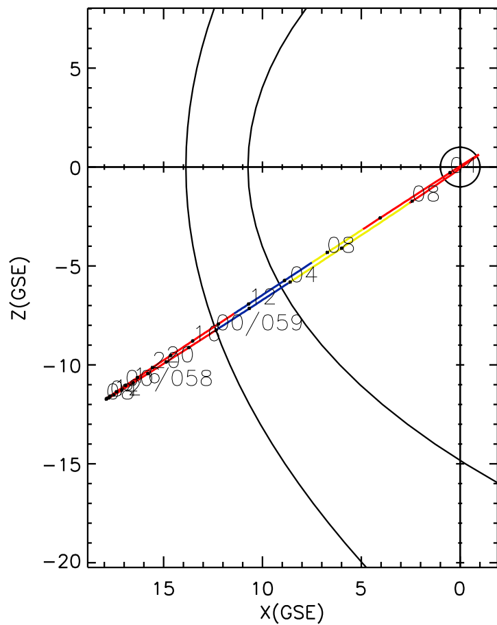
CLUSTER 2 orbit 2011 057 (02/26) 02:41 UT to 2011 059 (02/28) 08:56 UT
