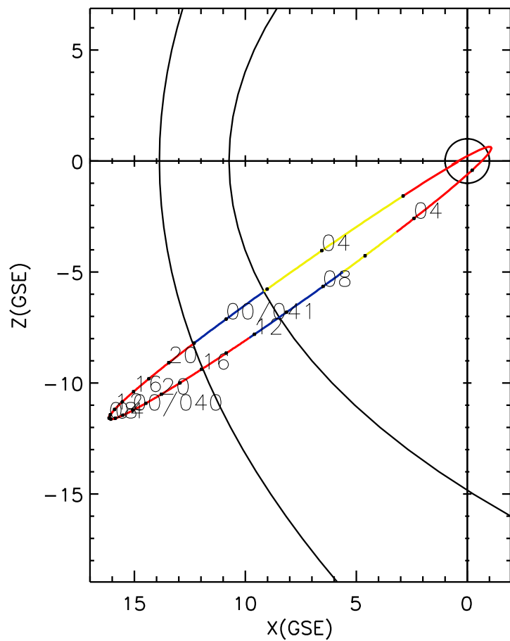
CLUSTER 2 orbit 2011 039 (02/08) 00:31 UT to 2011 041 (02/10) 06:51 UT
