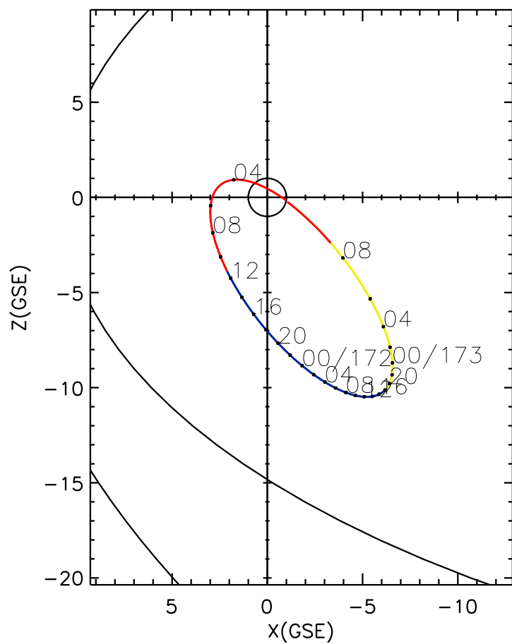
CLUSTER 2 orbit 2010 171 (06/20) 03:16 UT to 2010 173 (06/22) 09:31 UT
