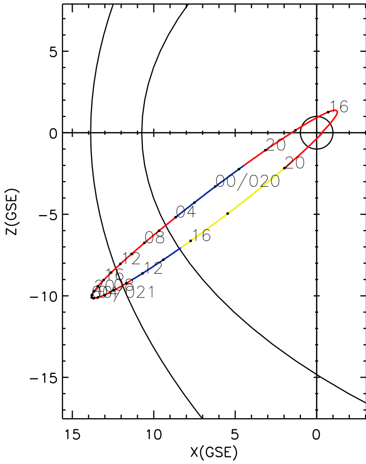
CLUSTER 2 orbit 2010 019 (01/19) 14:31 UT to 2010 021 (01/21) 20:51 UT
