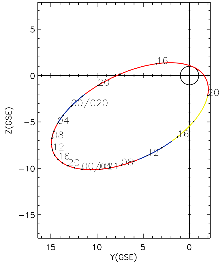
CLUSTER 2 orbit 2010 019 (01/19) 14:31 UT to 2010 021 (01/21) 20:51 UT
