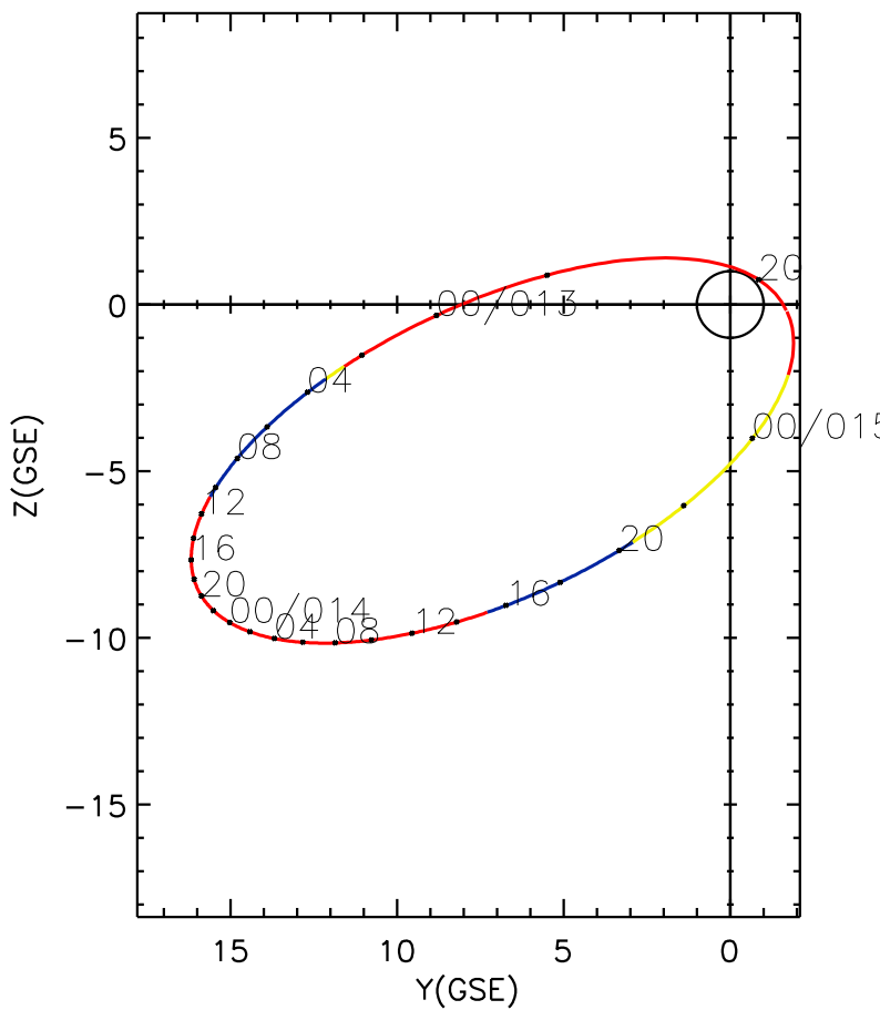
CLUSTER 2 orbit 2010 012 (01/12) 19:41 UT to 2010 015 (01/15) 01:56 UT
