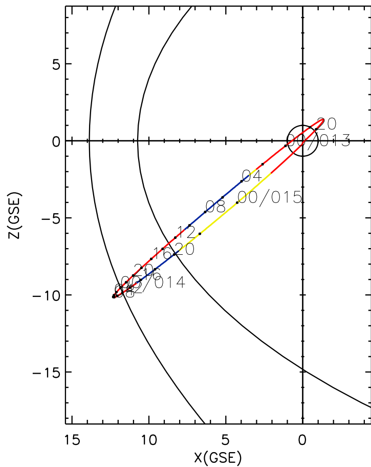
CLUSTER 2 orbit 2010 012 (01/12) 19:41 UT to 2010 015 (01/15) 01:56 UT
