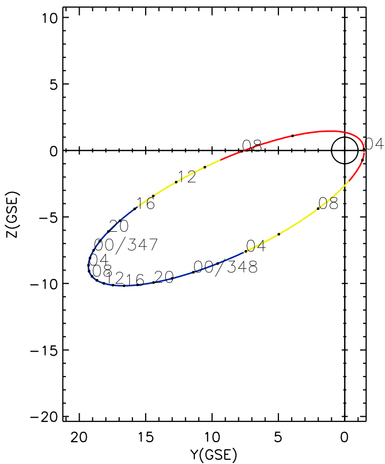
CLUSTER 2 orbit 2009 346 (12/12) 03:56 UT to 2009 348 (12/14) 10:11 UT
