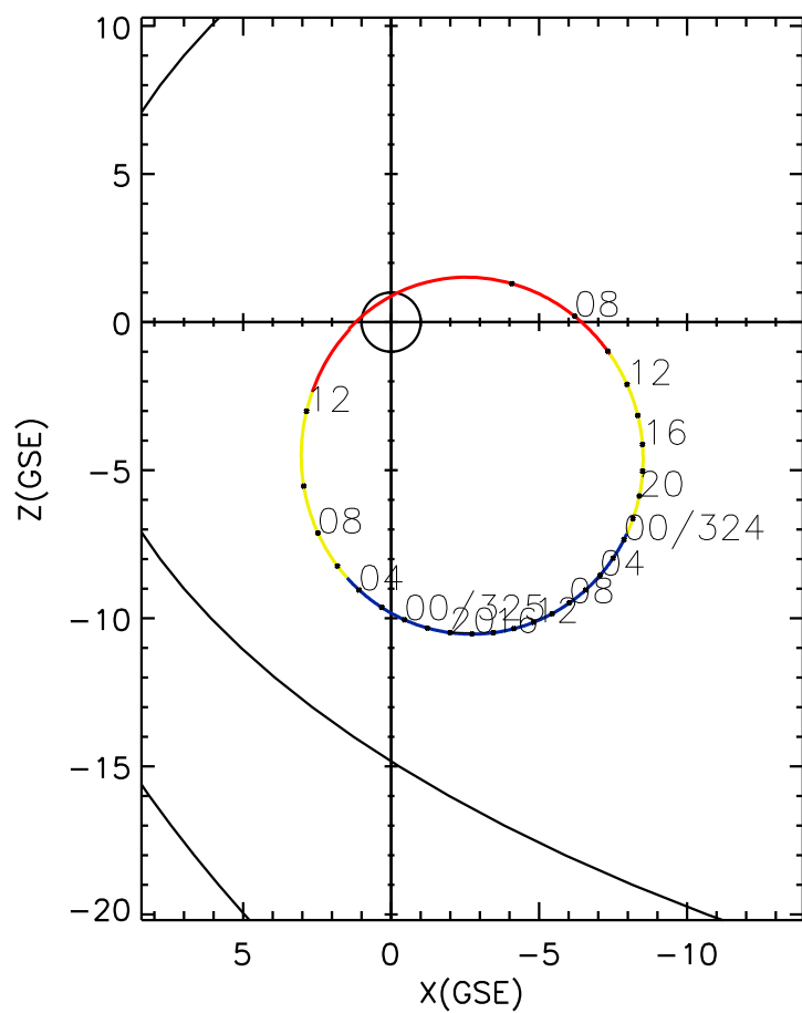
CLUSTER 2 orbit 2009 323 (11/19) 04:06 UT to 2009 325 (11/21) 13:11 UT
