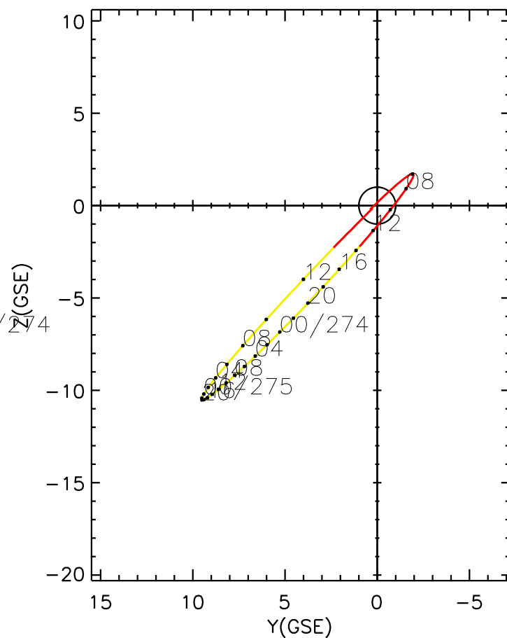
CLUSTER 2 orbit 2009 273 (09/30) 04:41 UT to 2009 275 (10/02) 13:51 UT
