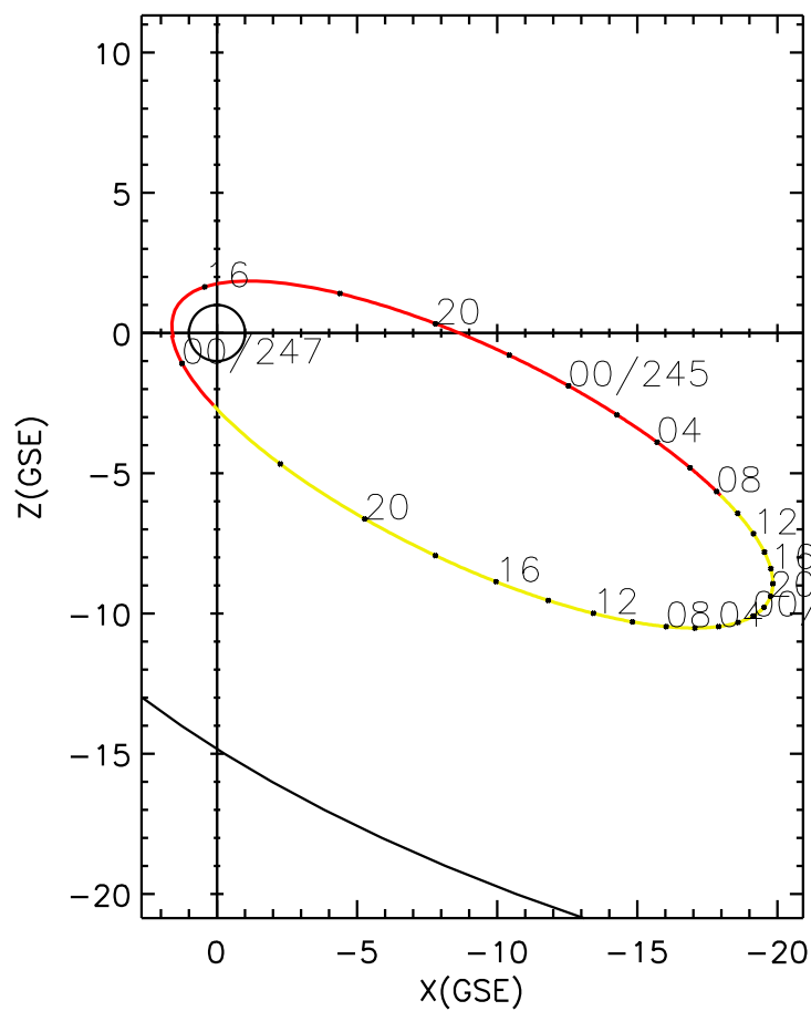
CLUSTER 2 orbit 2009 244 (09/01) 15:11 UT to 2009 247 (09/04) 00:21 UT
