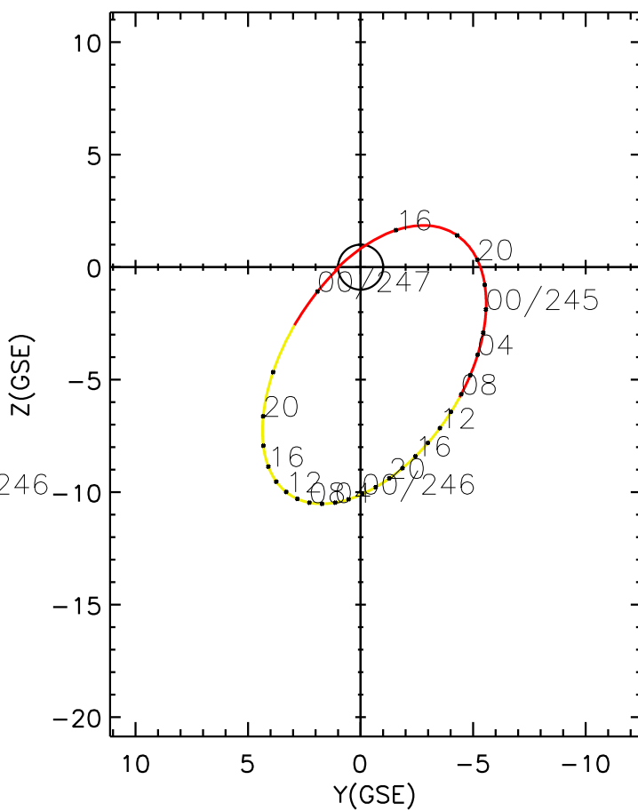
CLUSTER 2 orbit 2009 244 (09/01) 15:11 UT to 2009 247 (09/04) 00:21 UT
