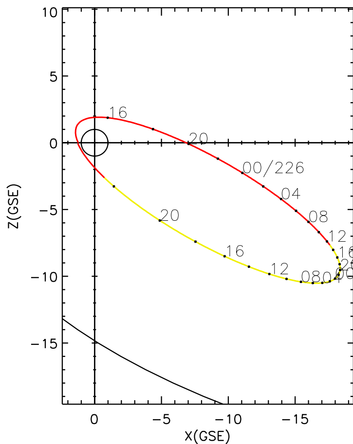
CLUSTER 2 orbit 2009 225 (08/13) 14:16 UT to 2009 227 (08/15) 23:21 UT
