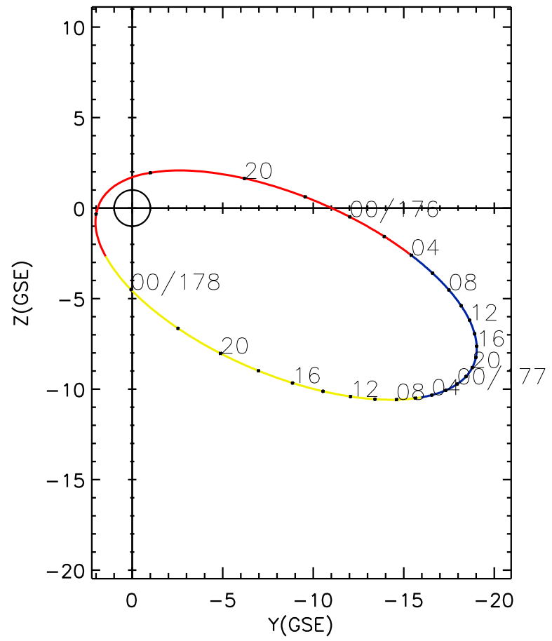
CLUSTER 2 orbit 2009 175 (06/24) 16:56 UT to 2009 178 (06/27) 02:06 UT
