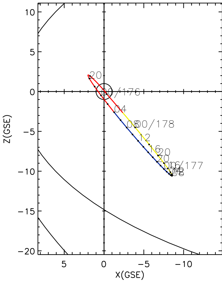
CLUSTER 2 orbit 2009 175 (06/24) 16:56 UT to 2009 178 (06/27) 02:06 UT
