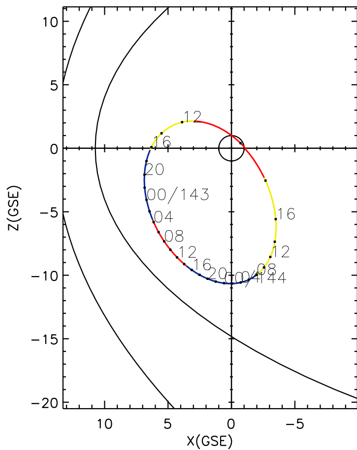
CLUSTER 2 orbit 2009 142 (05/22) 09:51 UT to 2009 144 (05/24) 18:56 UT
