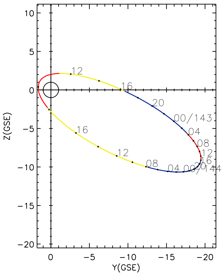
CLUSTER 2 orbit 2009 142 (05/22) 09:51 UT to 2009 144 (05/24) 18:56 UT
