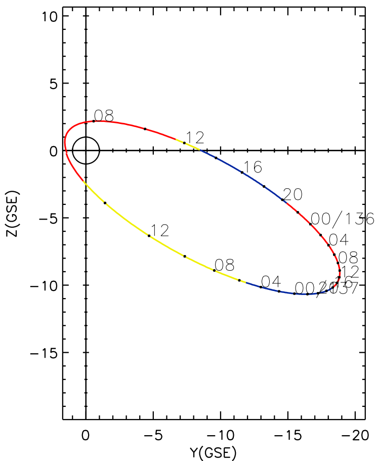
CLUSTER 2 orbit 2009 135 (05/15) 06:31 UT to 2009 137 (05/17) 15:36 UT
