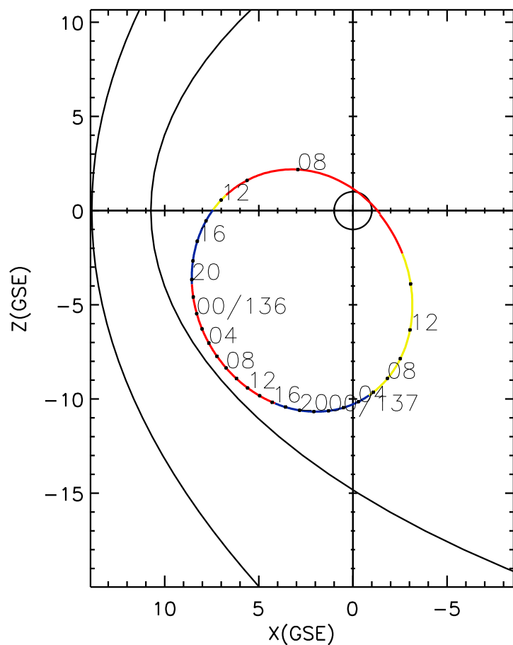
CLUSTER 2 orbit 2009 135 (05/15) 06:31 UT to 2009 137 (05/17) 15:36 UT
