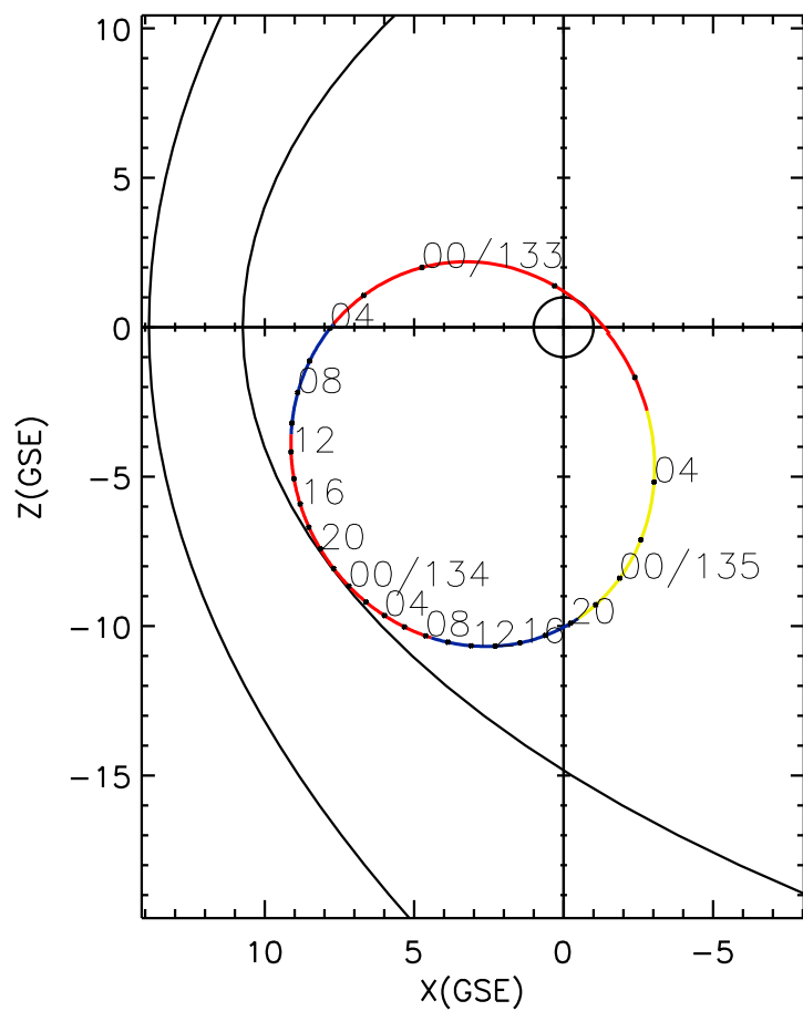
CLUSTER 2 orbit 2009 132 (05/12) 21:26 UT to 2009 135 (05/15) 06:31 UT
