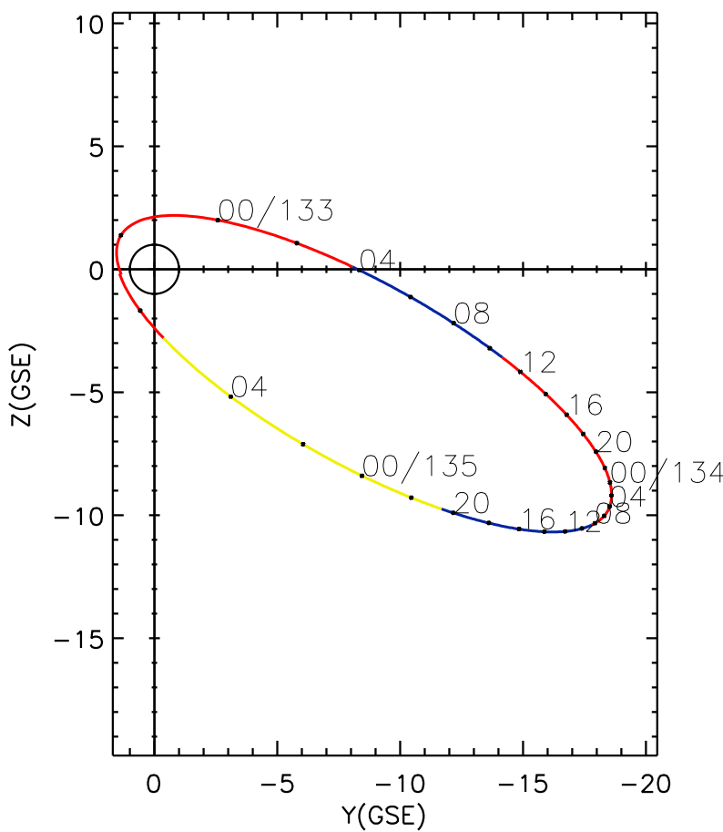
CLUSTER 2 orbit 2009 132 (05/12) 21:26 UT to 2009 135 (05/15) 06:31 UT
