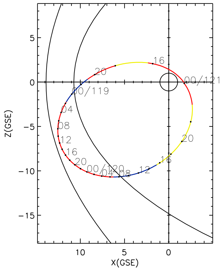
CLUSTER 2 orbit 2009 118 (04/28) 14:56 UT to 2009 121 (05/01) 00:01 UT
