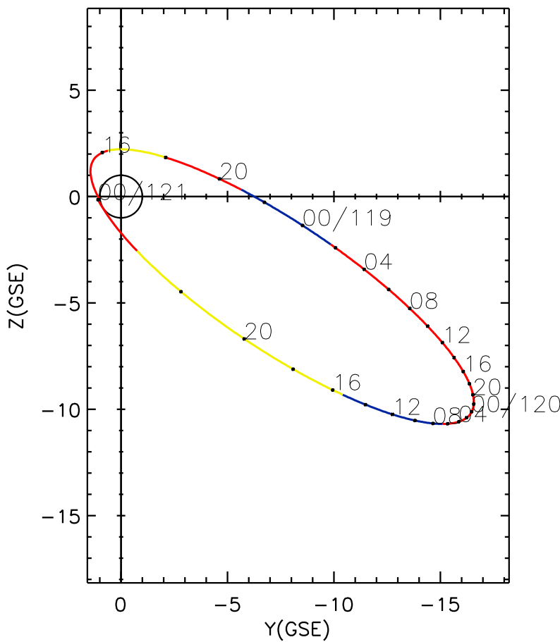
CLUSTER 2 orbit 2009 118 (04/28) 14:56 UT to 2009 121 (05/01) 00:01 UT
