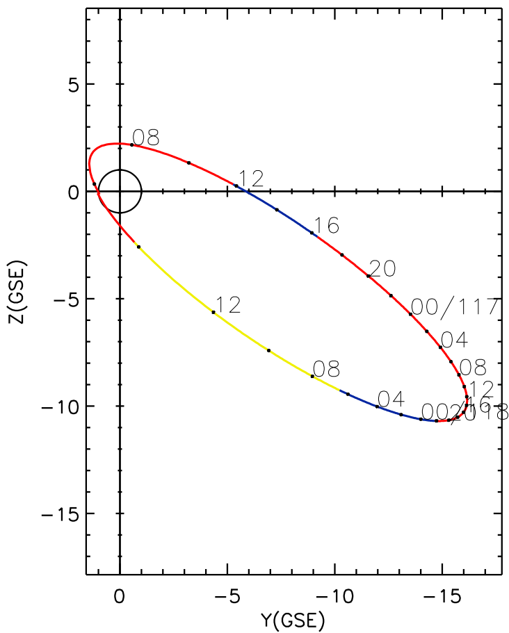
CLUSTER 2 orbit 2009 116 (04/26) 05:51 UT to 2009 118 (04/28) 14:56 UT
