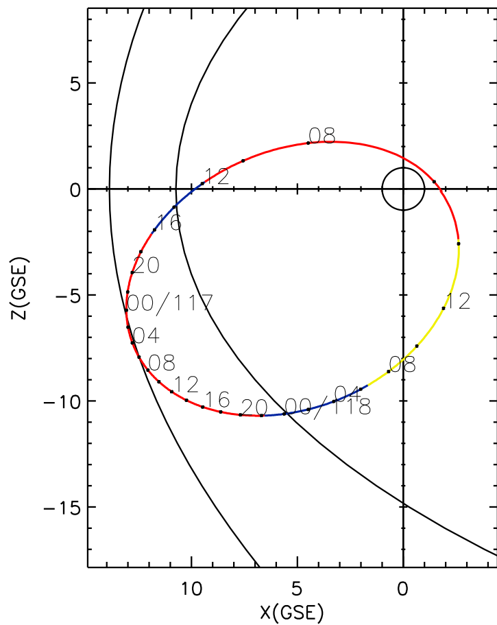
CLUSTER 2 orbit 2009 116 (04/26) 05:51 UT to 2009 118 (04/28) 14:56 UT
