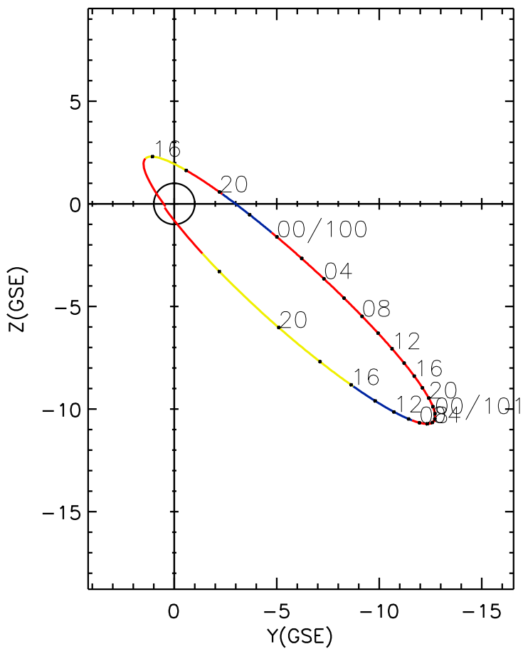
CLUSTER 2 orbit 2009 099 (04/09) 14:11 UT to 2009 101 (04/11) 23:16 UT
