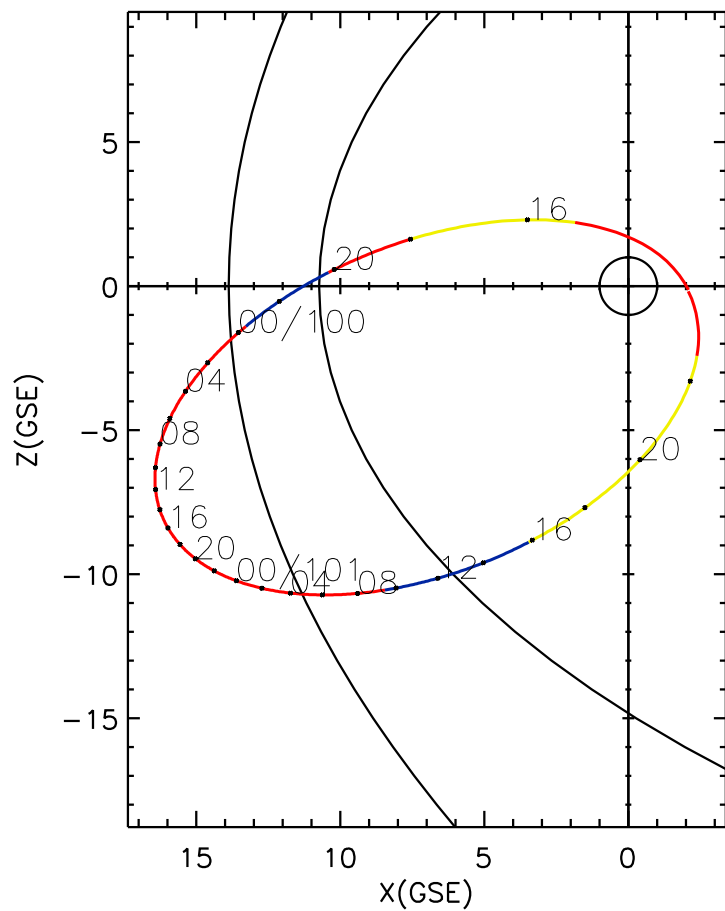
CLUSTER 2 orbit 2009 099 (04/09) 14:11 UT to 2009 101 (04/11) 23:16 UT
