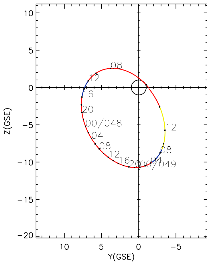
CLUSTER 2 orbit 2009 047 (02/16) 05:51 UT to 2009 049 (02/18) 14:56 UT
