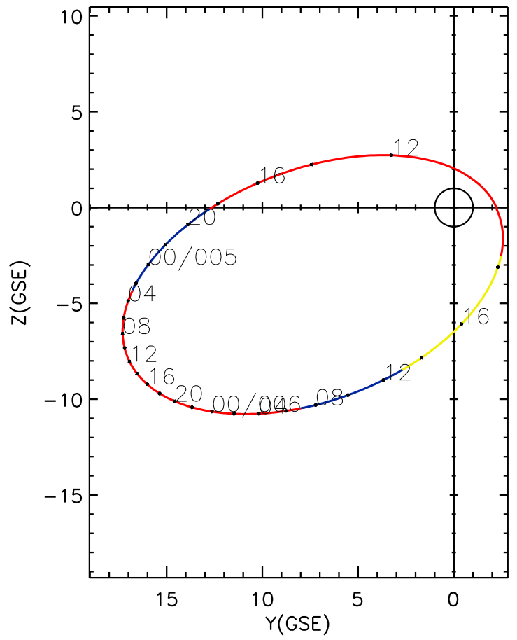
CLUSTER 2 orbit 2009 004 (01/04) 10:06 UT to 2009 006 (01/06) 19:11 UT
