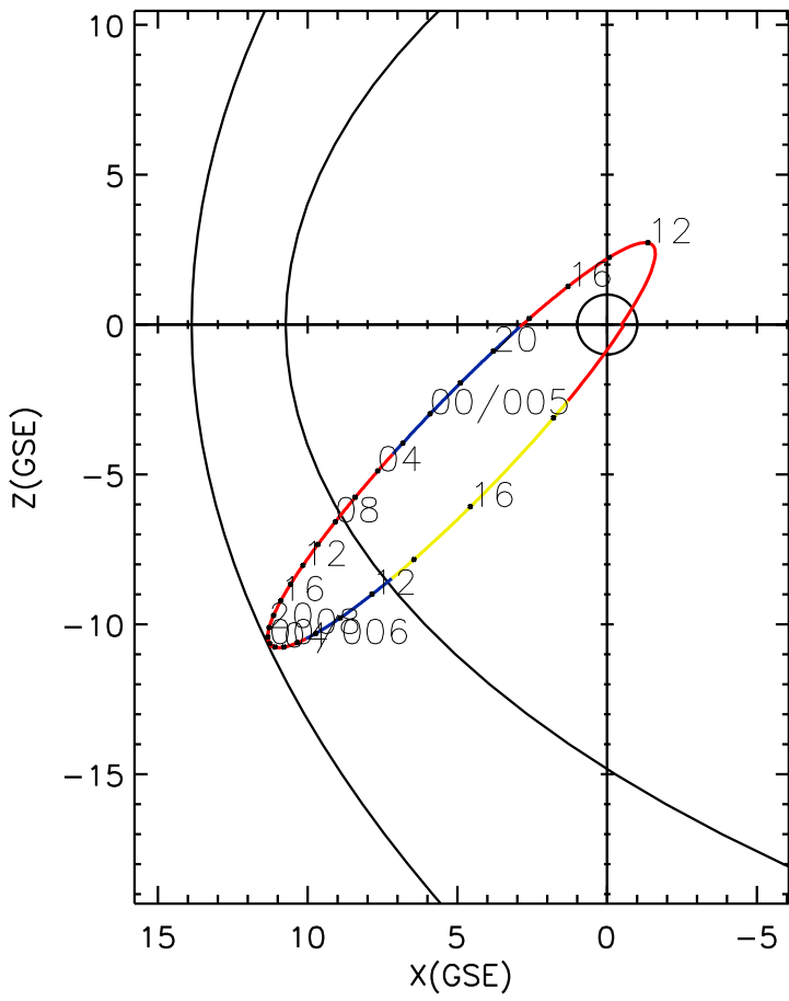
CLUSTER 2 orbit 2009 004 (01/04) 10:06 UT to 2009 006 (01/06) 19:11 UT
