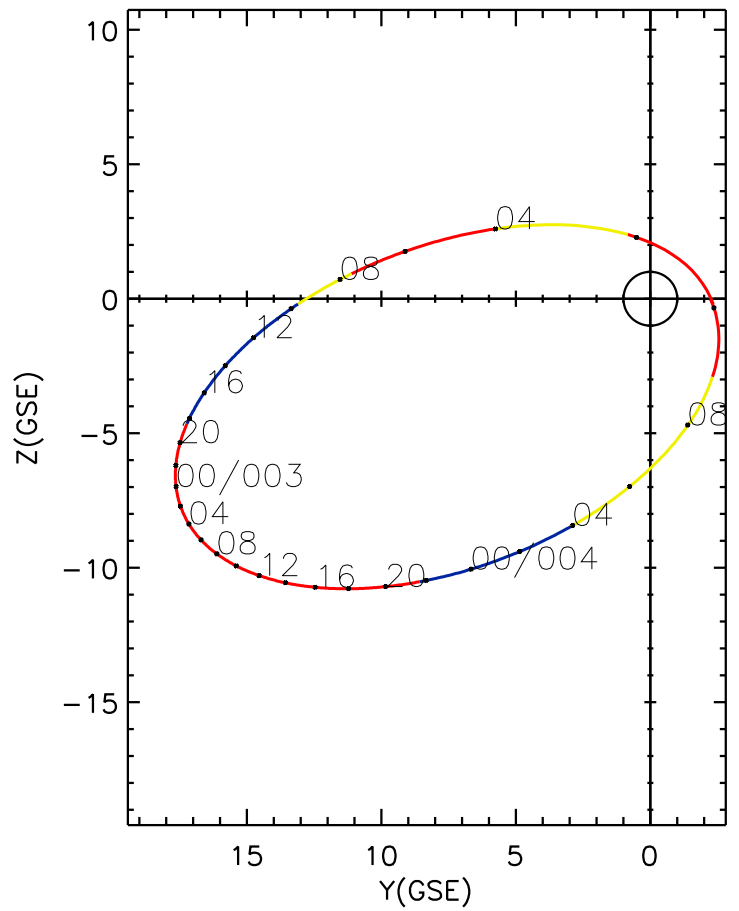
CLUSTER 2 orbit 2009 002 (01/02) 00:56 UT to 2009 004 (01/04) 10:06 UT
