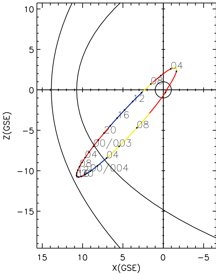
CLUSTER 2 orbit 2009 002 (01/02) 00:56 UT to 2009 004 (01/04) 10:06 UT
