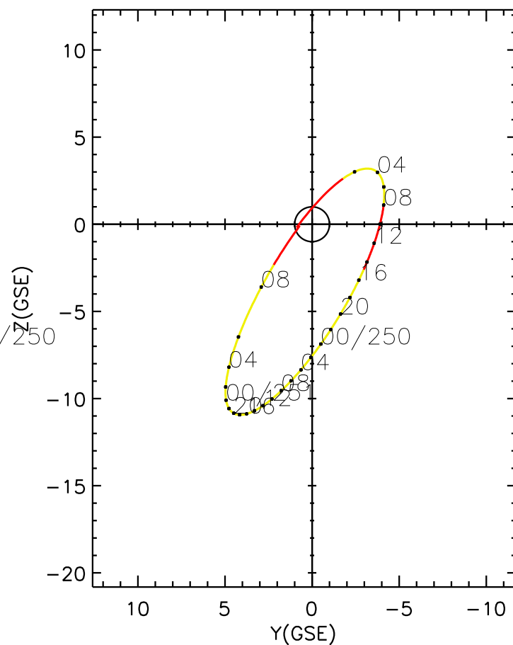
CLUSTER 2 orbit 2008 249 (09/05) 00:16 UT to 2008 251 (09/07) 09:26 UT
