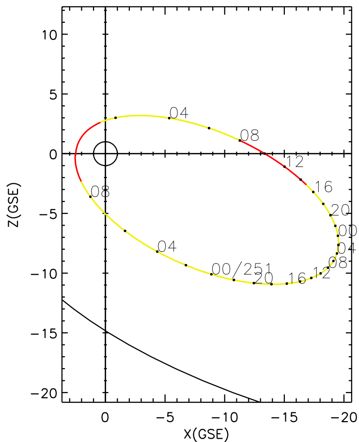
CLUSTER 2 orbit 2008 249 (09/05) 00:16 UT to 2008 251 (09/07) 09:26 UT
