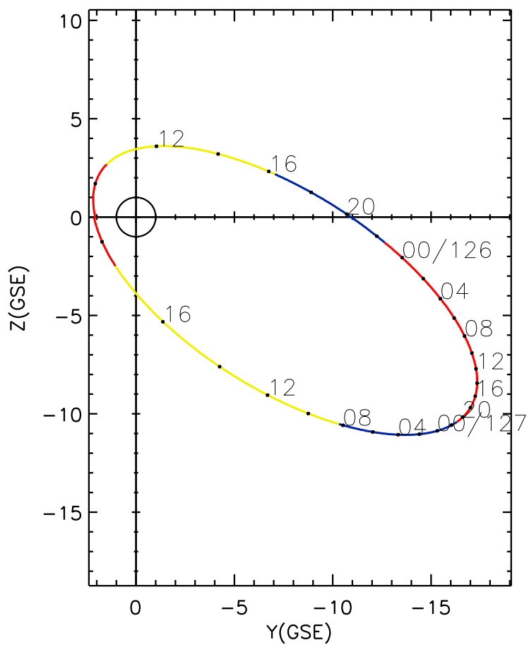
CLUSTER 2 orbit 2008 125 (05/04) 09:21 UT to 2008 127 (05/06) 18:26 UT
