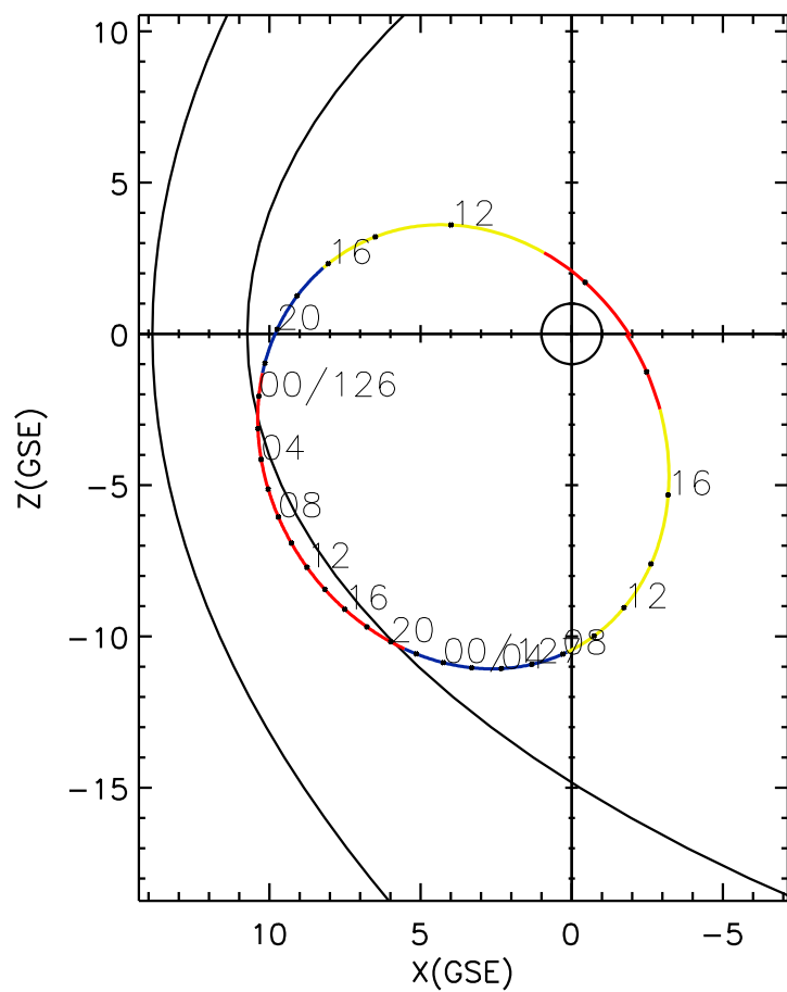
CLUSTER 2 orbit 2008 125 (05/04) 09:21 UT to 2008 127 (05/06) 18:26 UT
