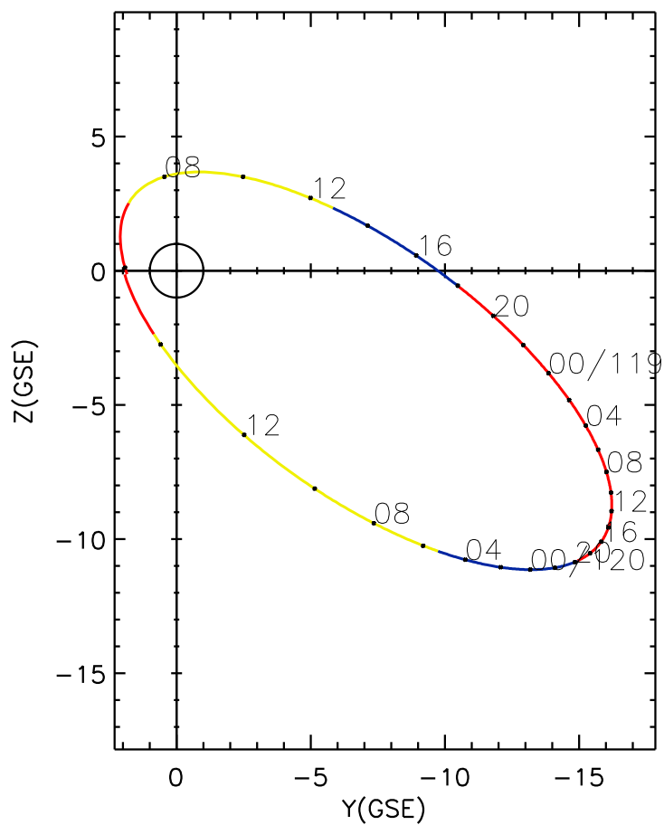
CLUSTER 2 orbit 2008 118 (04/27) 05:55 UT to 2008 120 (04/29) 15:00 UT
