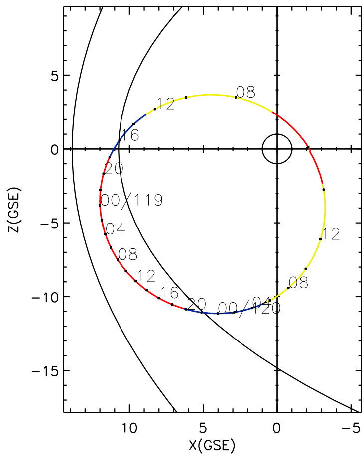
CLUSTER 2 orbit 2008 118 (04/27) 05:55 UT to 2008 120 (04/29) 15:00 UT
