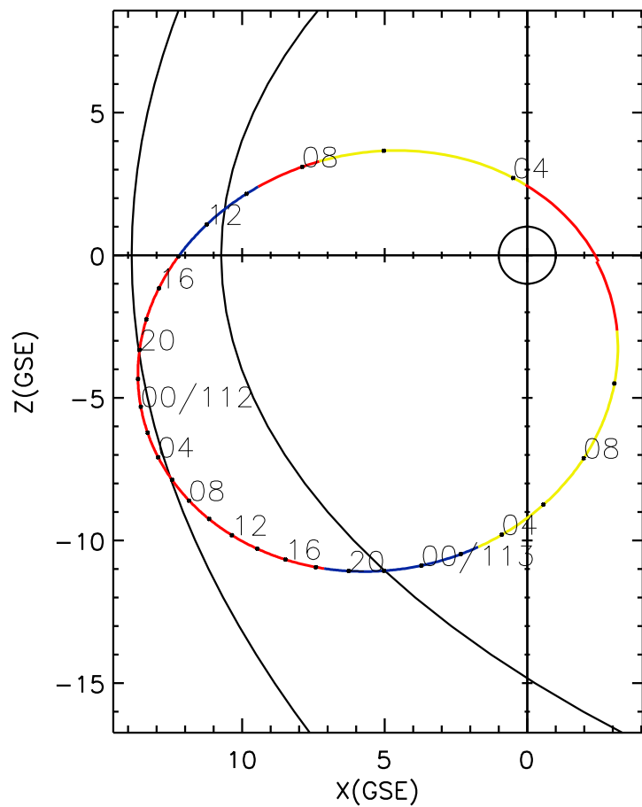
CLUSTER 2 orbit 2008 111 (04/20) 02:46 UT to 2008 113 (04/22) 11:51 UT
