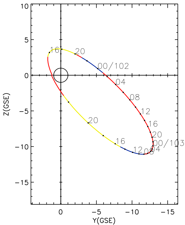
CLUSTER 2 orbit 2008 101 (04/10) 14:26 UT to 2008 103 (04/12) 23:31 UT
