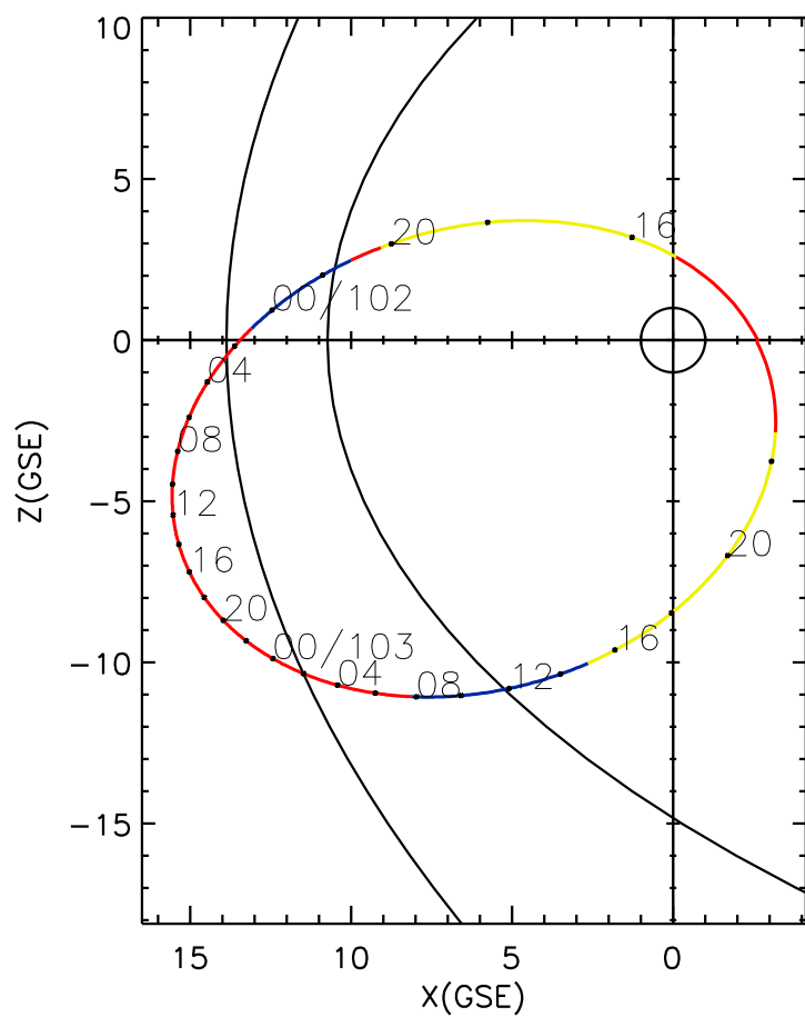
CLUSTER 2 orbit 2008 101 (04/10) 14:26 UT to 2008 103 (04/12) 23:31 UT
