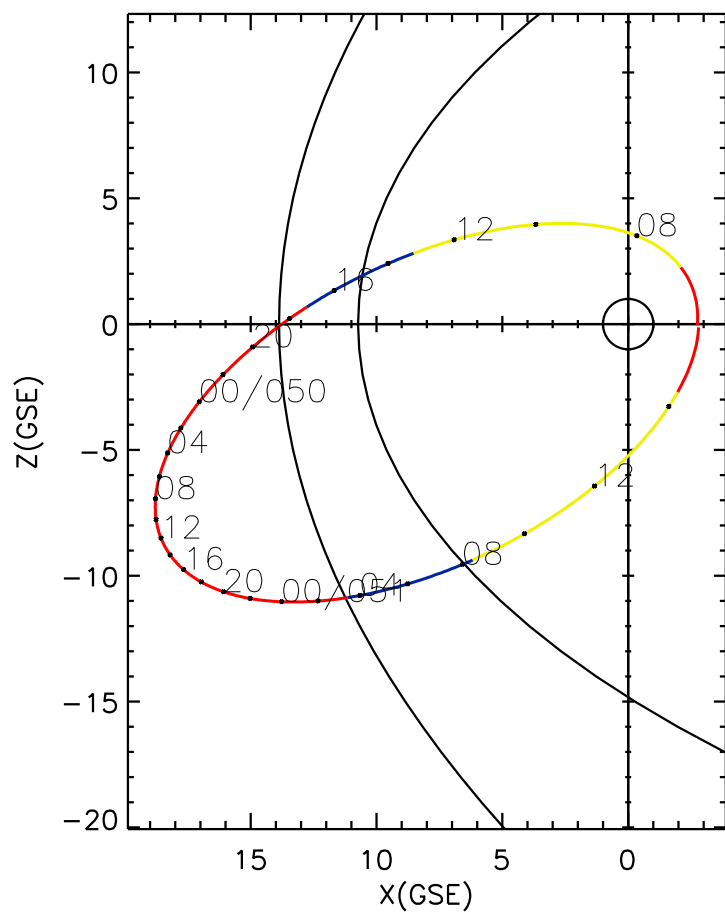
CLUSTER 2 orbit 2008 049 (02/18) 06:11 UT to 2008 051 (02/20) 15:16 UT
