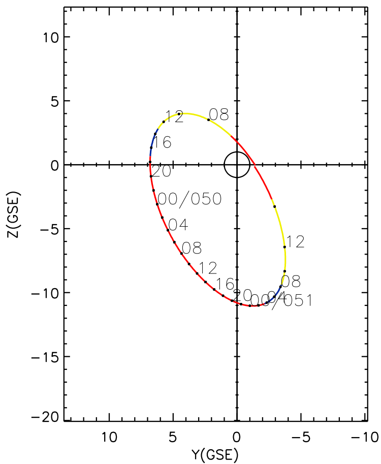
CLUSTER 2 orbit 2008 049 (02/18) 06:11 UT to 2008 051 (02/20) 15:16 UT
