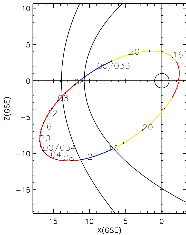
CLUSTER 2 orbit 2008 032 (02/01) 14:31 UT to 2008 034 (02/03) 23:31 UT
