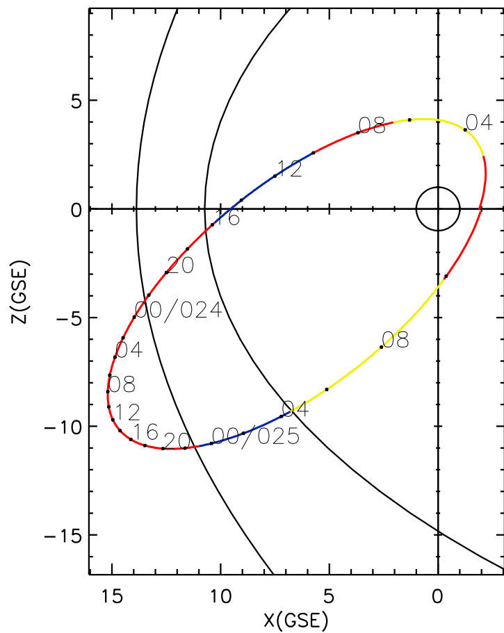
CLUSTER 2 orbit 2008 023 (01/23) 02:06 UT to 2008 025 (01/25) 11:11 UT
