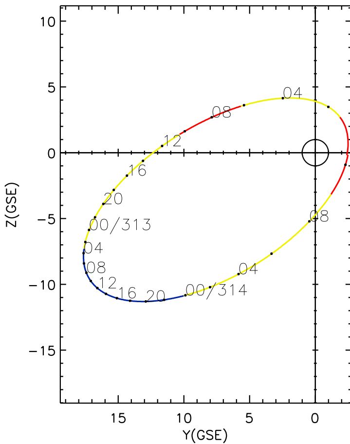
CLUSTER 2 orbit 2007 312 (11/08) 00:16 UT to 2007 314 (11/10) 10:16 UT
