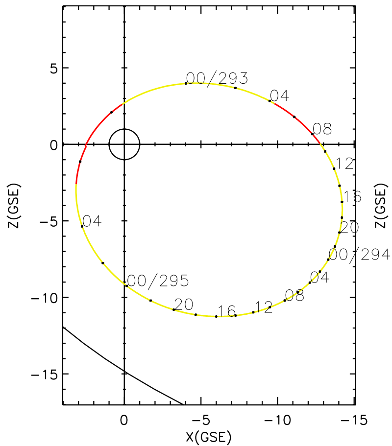
CLUSTER 2 orbit 2007 292 (10/19) 21:11 UT to 2007 295 (10/22) 06:21 UT
