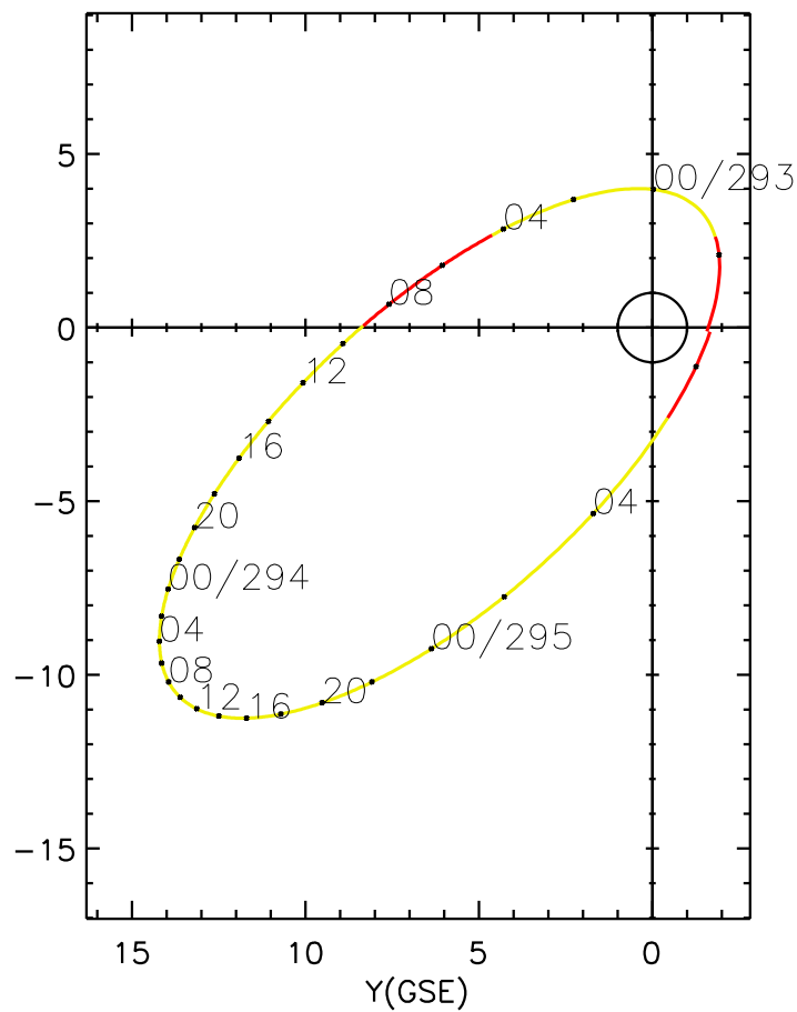
CLUSTER 2 orbit 2007 292 (10/19) 21:11 UT to 2007 295 (10/22) 06:21 UT
