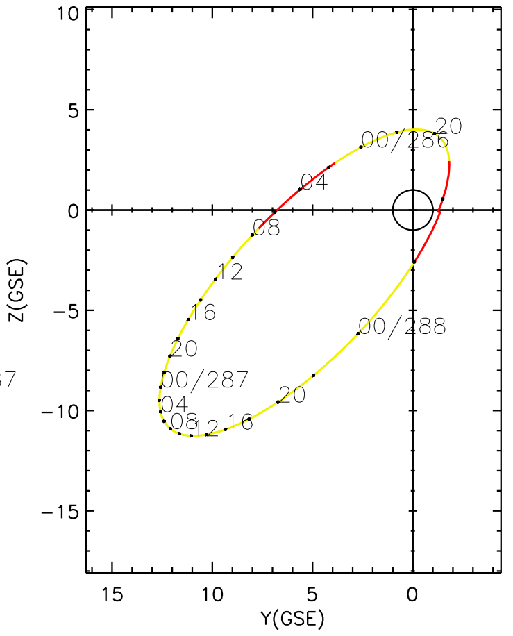
CLUSTER 2 orbit 2007 285 (10/12) 17:46 UT to 2007 288 (10/15) 02:56 UT
