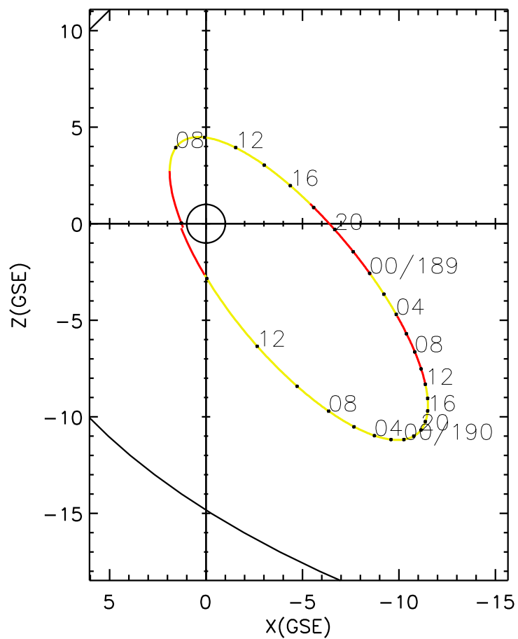
CLUSTER 2 orbit 2007 188 (07/07) 05:55 UT to 2007 190 (07/09) 15:00 UT
