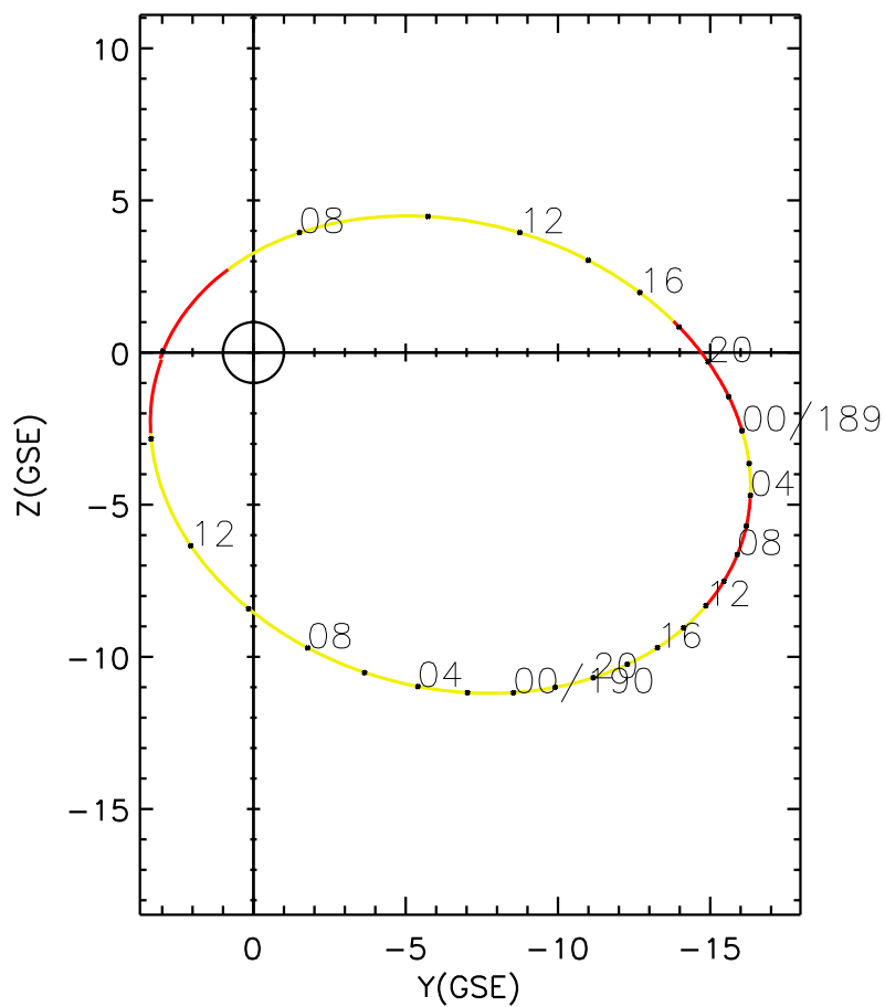
CLUSTER 2 orbit 2007 188 (07/07) 05:55 UT to 2007 190 (07/09) 15:00 UT
