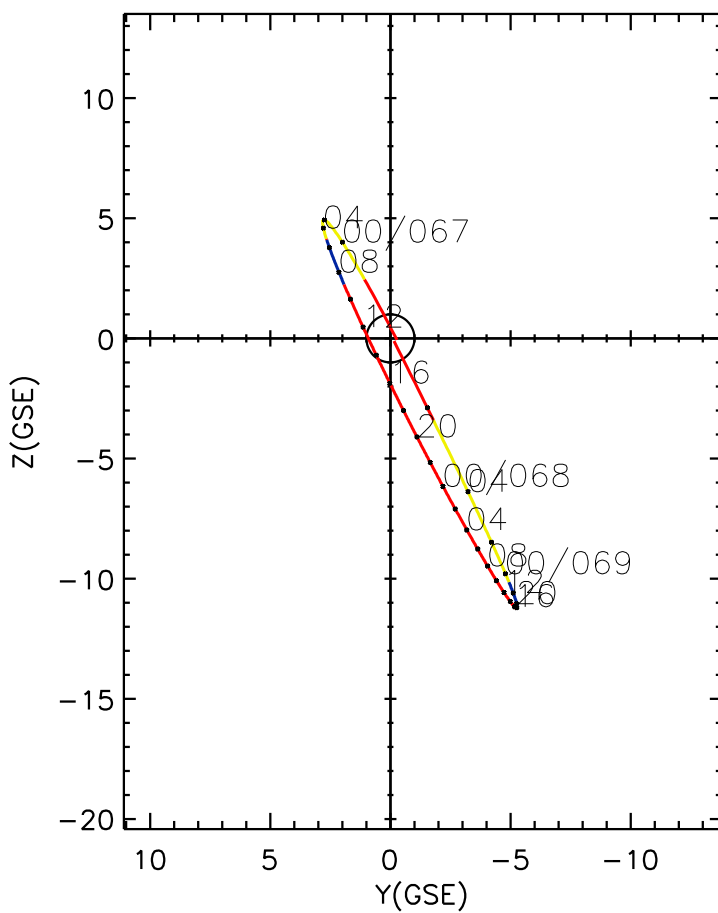
CLUSTER 2 orbit 2007 066 (03/07) 22:01 UT to 2007 069 (03/10) 07:06 UT
