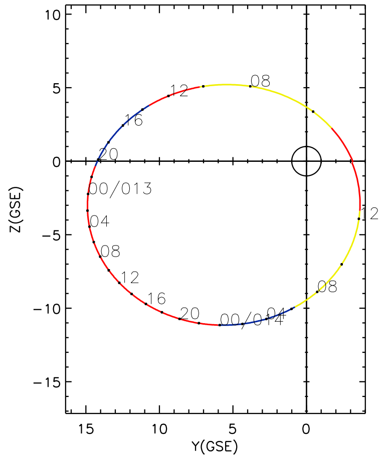
CLUSTER 2 orbit 2007 012 (01/12) 04:31 UT to 2007 014 (01/14) 13:36 UT
