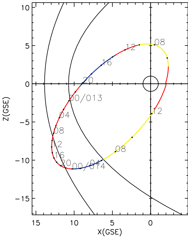
CLUSTER 2 orbit 2007 012 (01/12) 04:31 UT to 2007 014 (01/14) 13:36 UT
