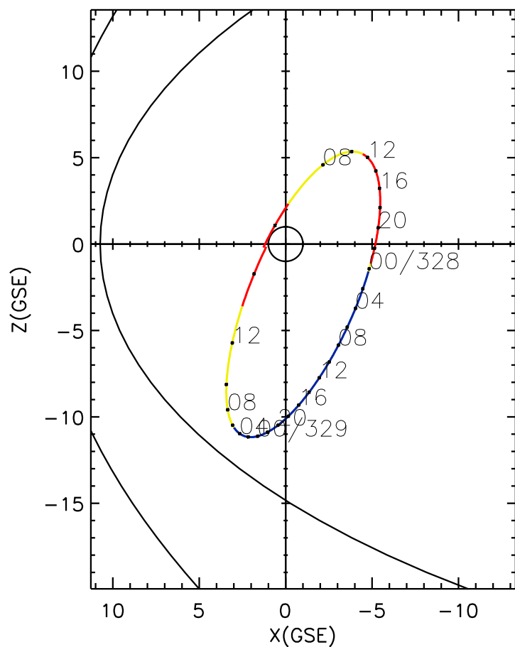
CLUSTER 2 orbit 2006 327 (11/23) 05:31 UT to 2006 329 (11/25) 14:36 UT
