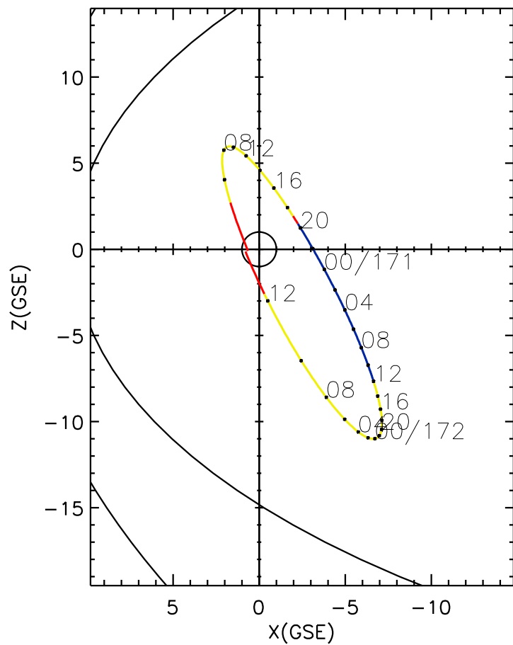
CLUSTER 2 orbit 2006 170 (06/19) 04:06 UT to 2006 172 (06/21) 13:11 UT
