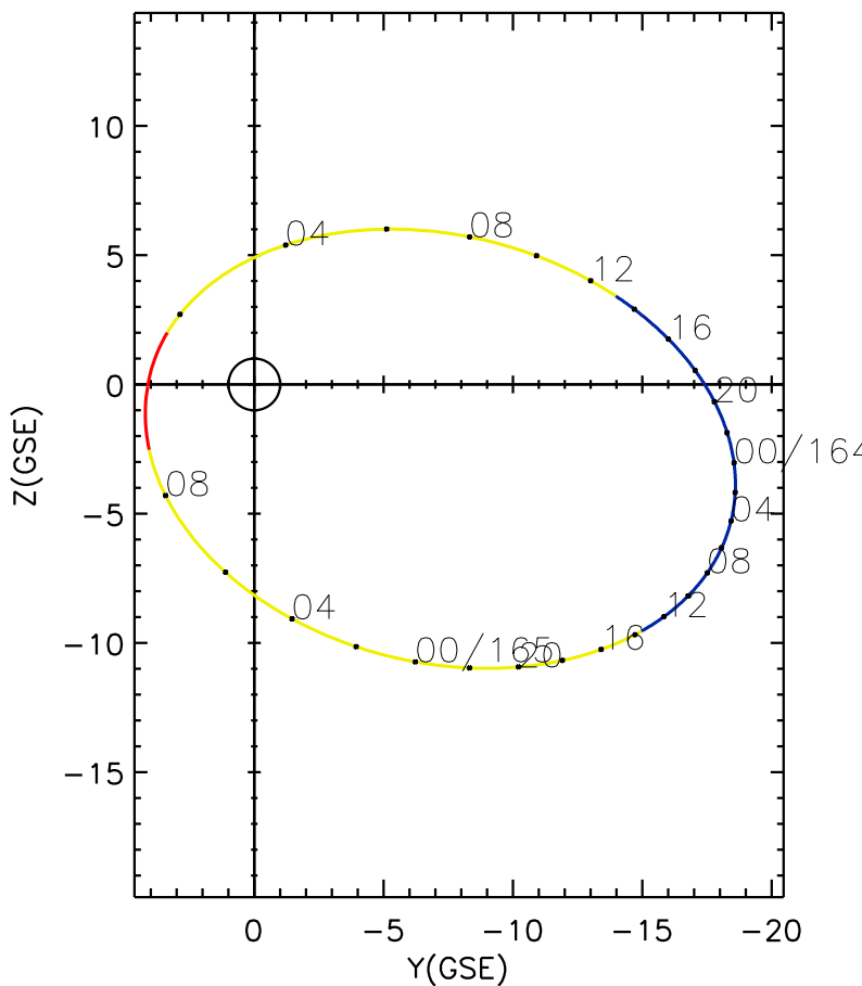
CLUSTER 2 orbit 2006 163 (06/12) 00:51 UT to 2006 165 (06/14) 09:51 UT
