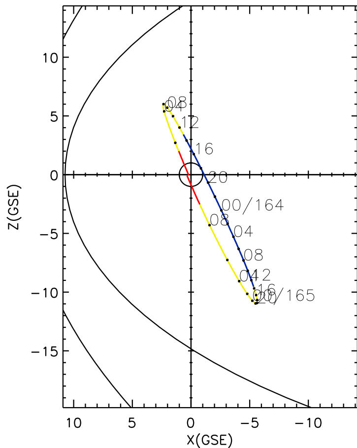
CLUSTER 2 orbit 2006 163 (06/12) 00:51 UT to 2006 165 (06/14) 09:51 UT
