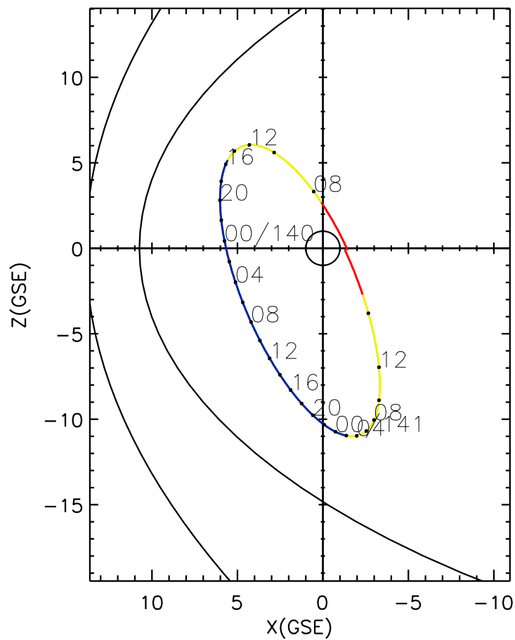
CLUSTER 2 orbit 2006 139 (05/19) 06:31 UT to 2006 141 (05/21) 15:36 UT
