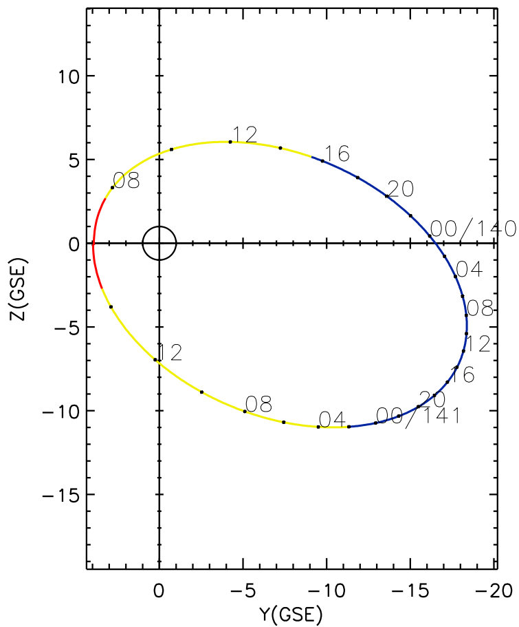
CLUSTER 2 orbit 2006 139 (05/19) 06:31 UT to 2006 141 (05/21) 15:36 UT
