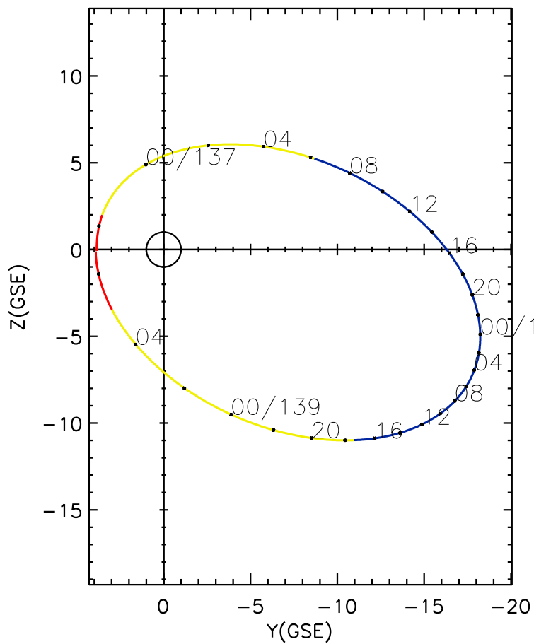
CLUSTER 2 orbit 2006 136 (05/16) 21:26 UT to 2006 139 (05/19) 06:31 UT
