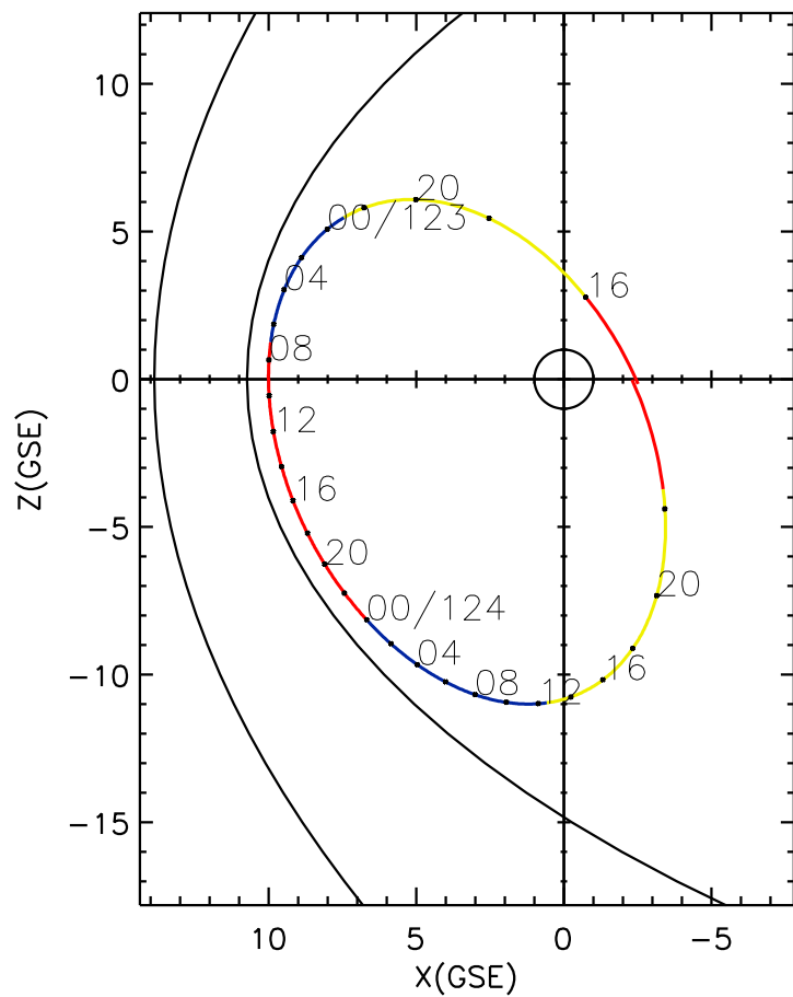
CLUSTER 2 orbit 2006 122 (05/02) 14:46 UT to 2006 124 (05/04) 23:56 UT
