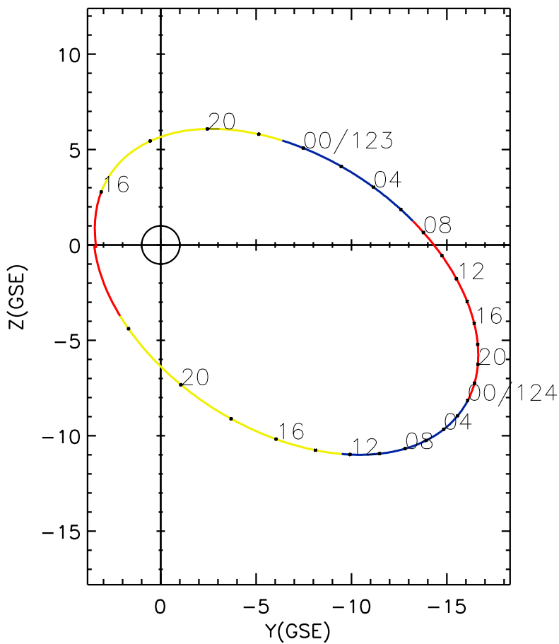
CLUSTER 2 orbit 2006 122 (05/02) 14:46 UT to 2006 124 (05/04) 23:56 UT
