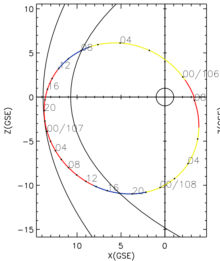
CLUSTER 2 orbit 2006 105 (04/15) 23:01 UT to 2006 108 (04/18) 08:06 UT
